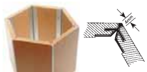
AP8017 - 120° Outside Corner
